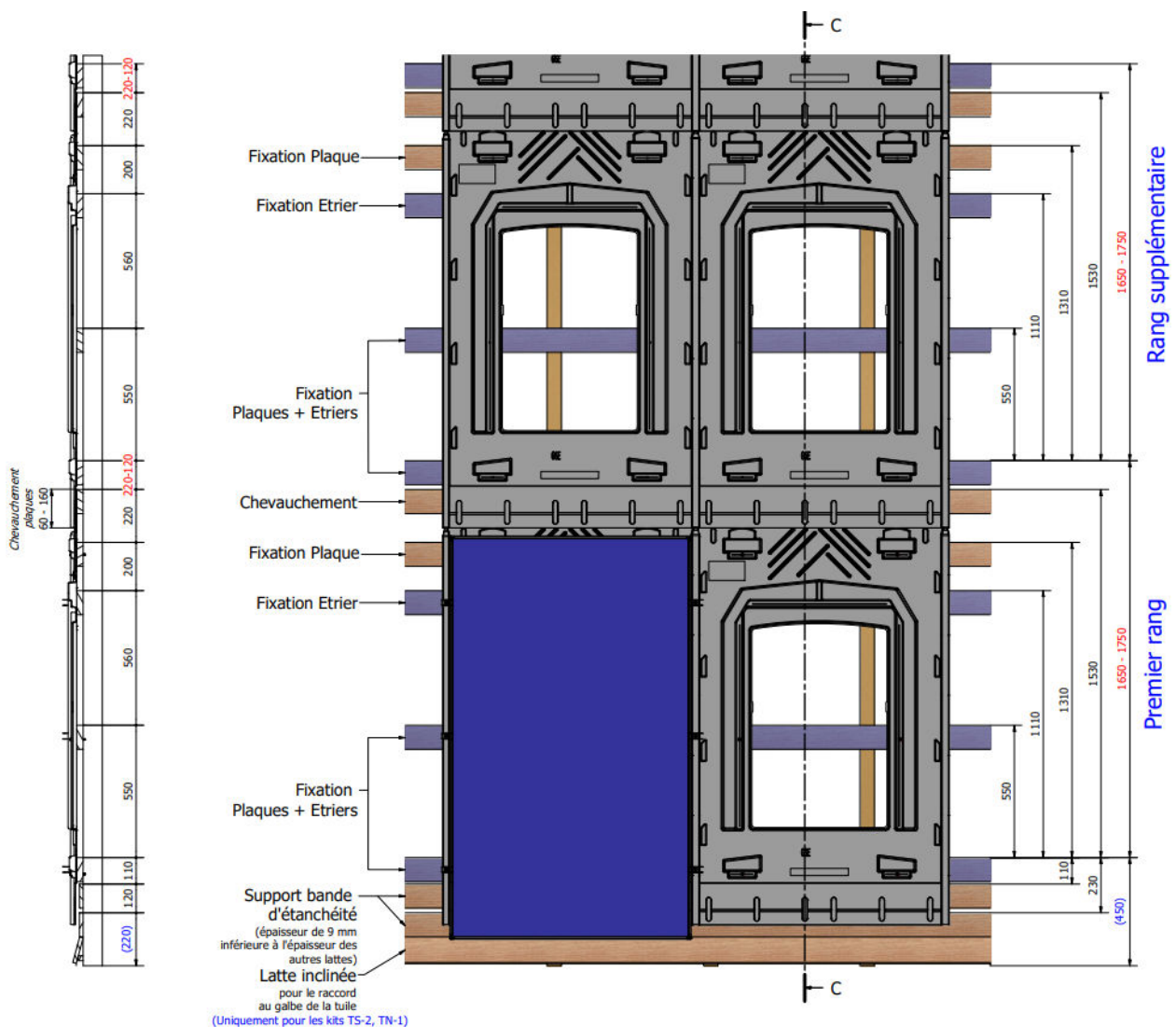
Figure 16 – Support et recouvrement des plaques polypropylène – plaques 1640_xxx
