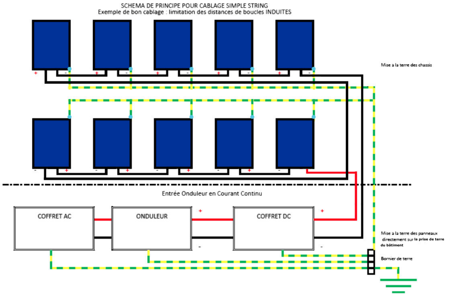
Figure 13 – Principe de câblage
