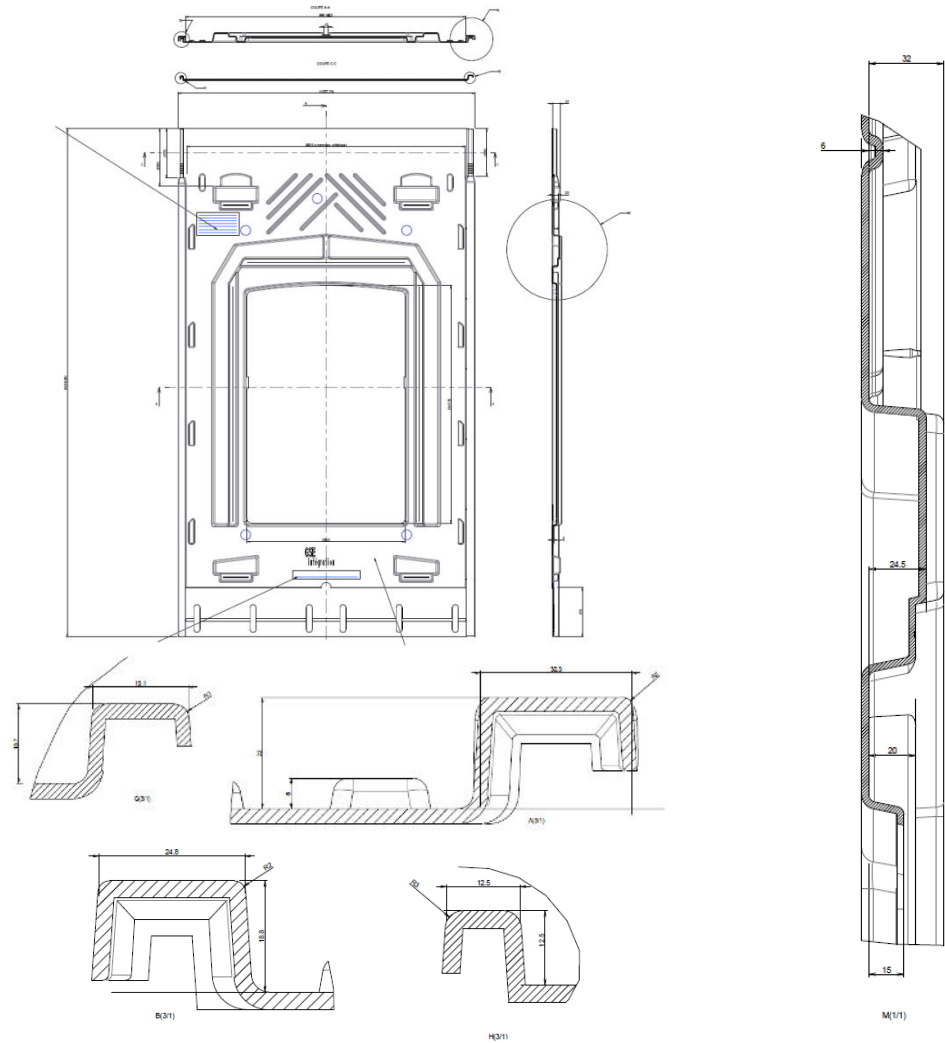
Figure 2 – Plaque polypropylène (exemple format 1640_992)
