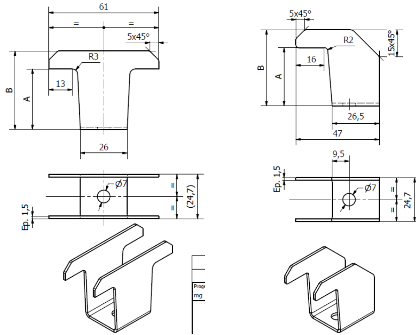
Figure 3 – Étriers
