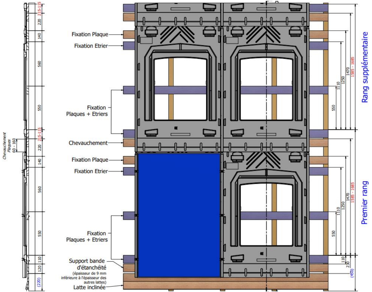
Figure 17 – Support et recouvrement des plaques polypropylène – plaque 1575_1046
