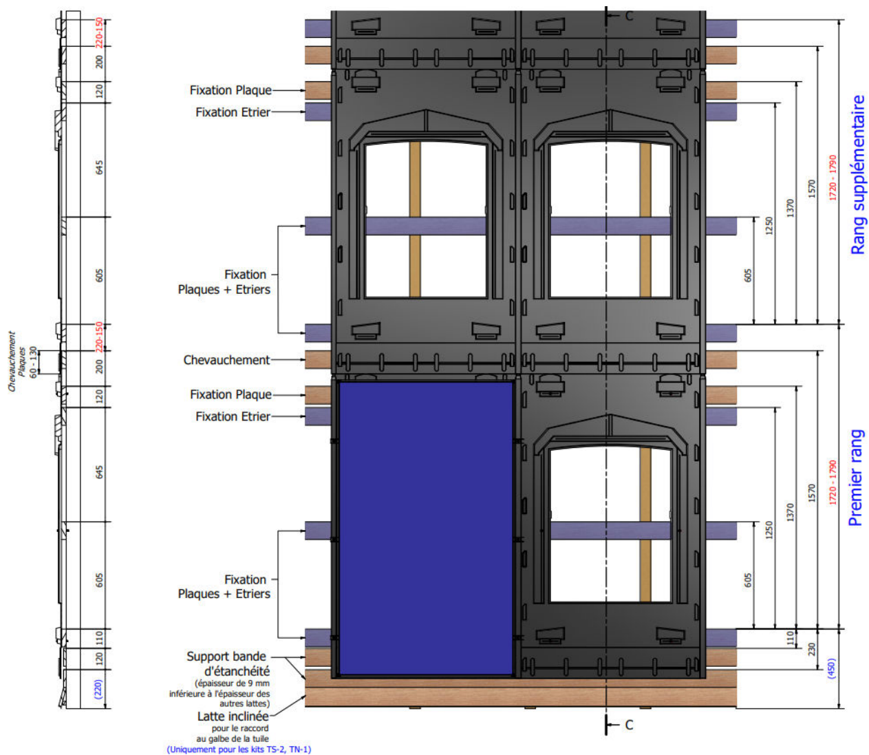
Figure 18 – Support et recouvrement des plaques polypropylène – plaques 1710_xxx
