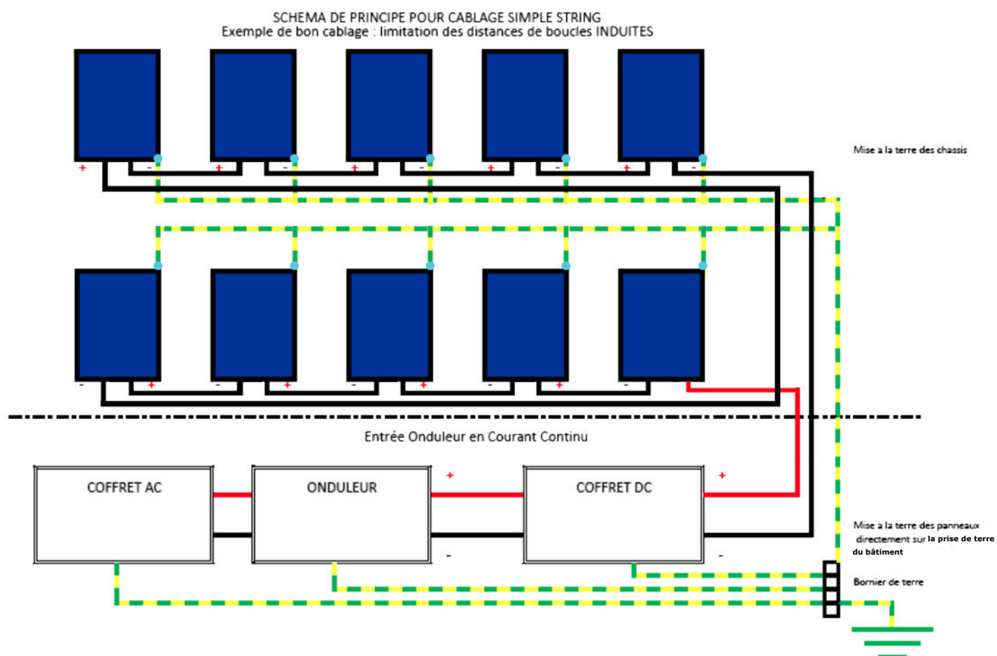
Figure 13 – Principe de câblage
