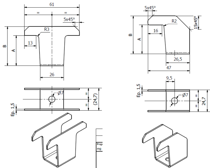
Figure 3 – Étriers
